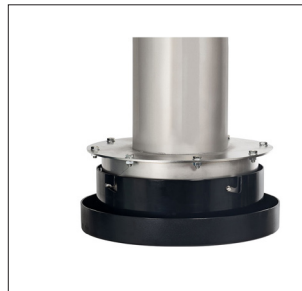
Longopac Fill Mini A cassette holder designed for mounting to a machine with vertical discharge (0-90°). Max. diameter 250.
